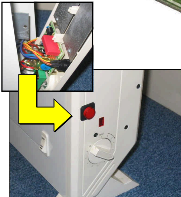
Illuminated pushbutton
