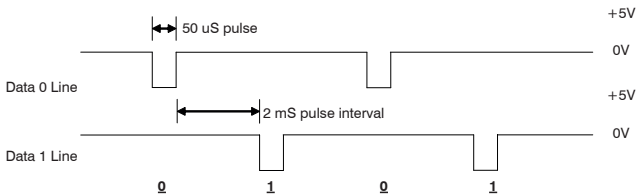
Diagram of The Wiegand Protocol Timing and Its Electrical Manner
